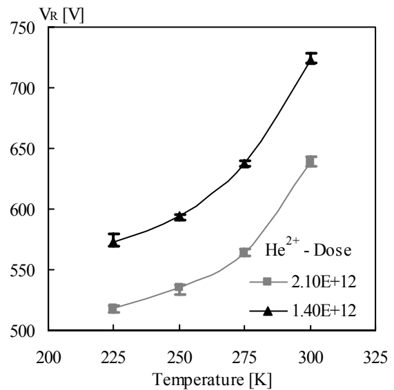
Fig. 14: Temperature dependence of reverse voltage for an avalanche current of 30\text{A/cm}^2 (helium-radiated samples)
